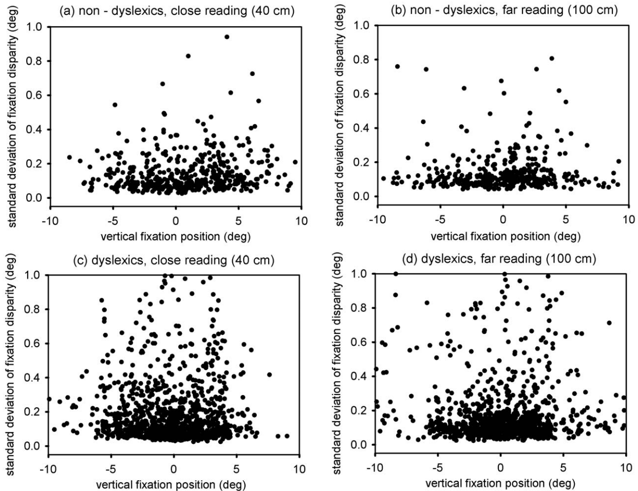
Figure 5. The different plots show the standard deviation of fixation disparity as a function of vertical fixation position (deg), i.e., as a function of the vertical position within the text at which the children looked at. The two lefthand plots show data for the close reading while the two righthand plots show data for the far reading. Upper plots (a & b) are those for non-dyslexic children (N=7) while the lower plots (c & d) show data of the dyslexic children (N=13). doi:10.1371/journal.pone.0018694.g005
