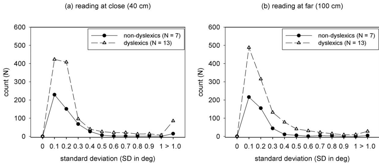
Figure 3. Histogram of the standard deviation (SD in deg) of fixation disparity measured while the children read the text at (a) close reading distance (40 cm) and at (b) far reading distance (100 cm); the plots show the data for non-dyslexic (dots) and dyslexic children (triangles), respectively. doi:10.1371/journal.pone.0018694.g003
