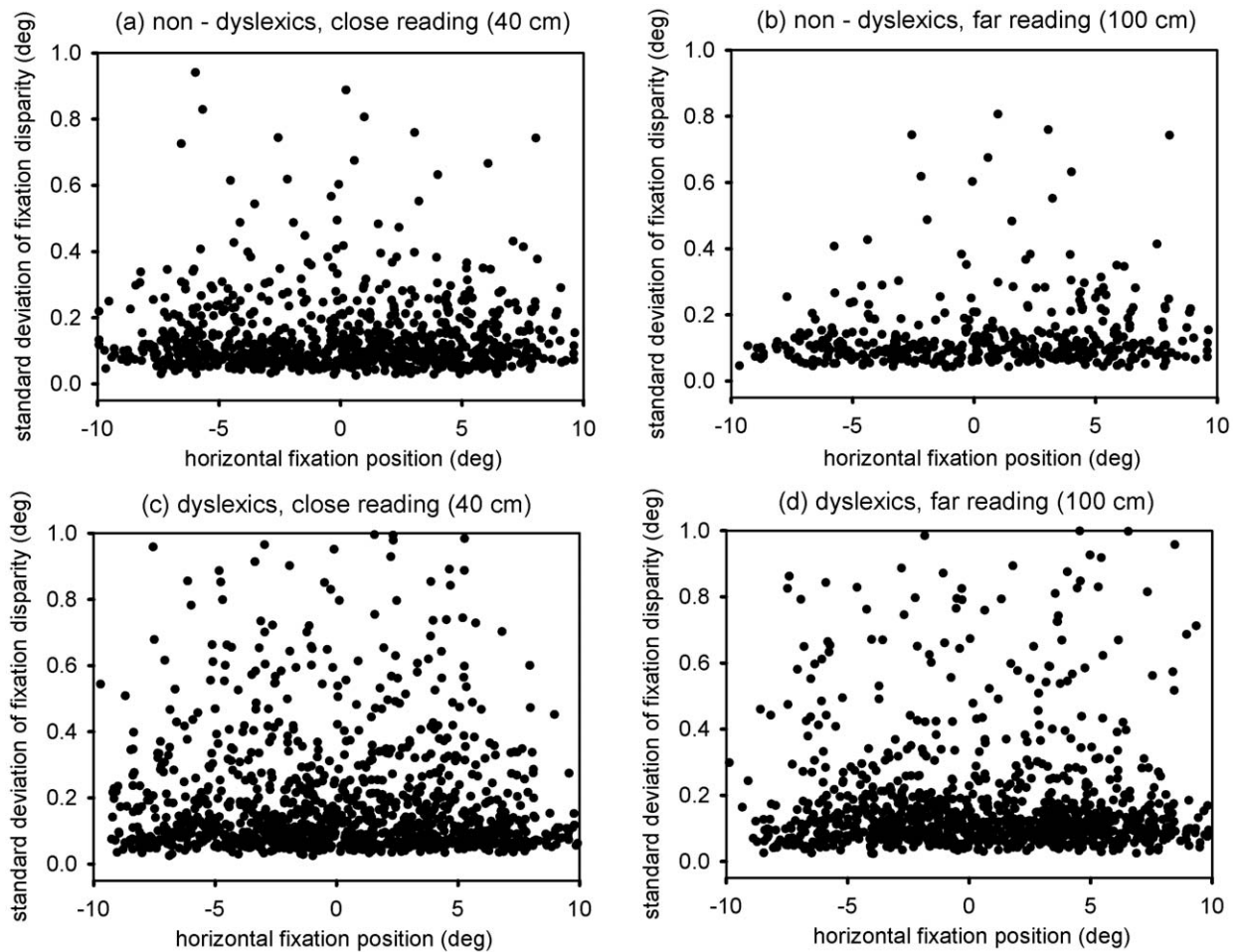
Figure 4. The different plots show the standard deviation of fixation disparity as a function of horizontal fixation position (deg), i.e., as a function of the horizontal position within the text at which the children looked at. The two lefthand plots show data for the close reading while the two righthand plots show data for the far reading. Upper plots (a & b) are those for non-dyslexic children (N=7) while the lower plots (c & d) show data of the dyslexic children (N=13). doi:10.1371/journal.pone.0018694.g004
