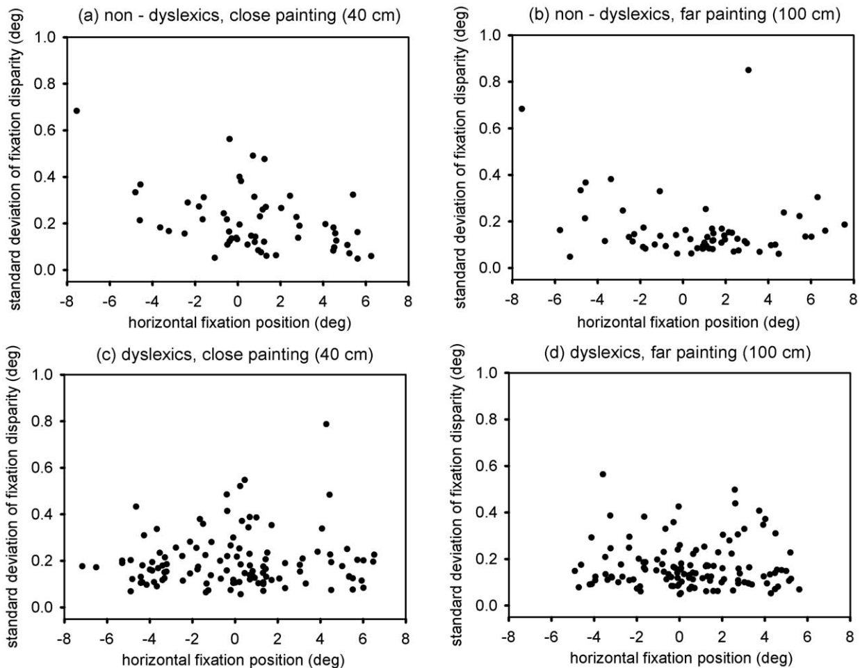
Figure 6. The different plots show the standard deviation of fixation disparity as a function of horizontal fixation position (deg), i.e., as a function of the horizontal position within the painting which the children looked at. The two lefthand plots show data for a close viewing distance while the two righthand plots show data for the far viewing distance, respectively. Upper plots (a & b) are those for non-dyslexic children (N=2) while the lower plots (c & d) show data of the dyslexic children (N=3). doi:10.1371/journal.pone.0018694.g006
